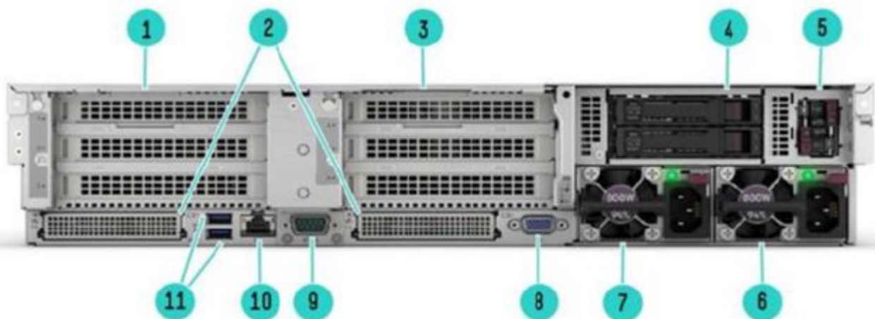
HPE ProLiant DL385 Gen11 - Rear View
